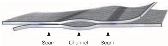
Prefabricated pipe boots, flashings and details are seamed with hot air guns. Quality control testing is provided by means of high pressure air lance testing.
