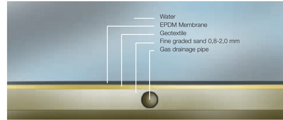
Reservoir construction.
